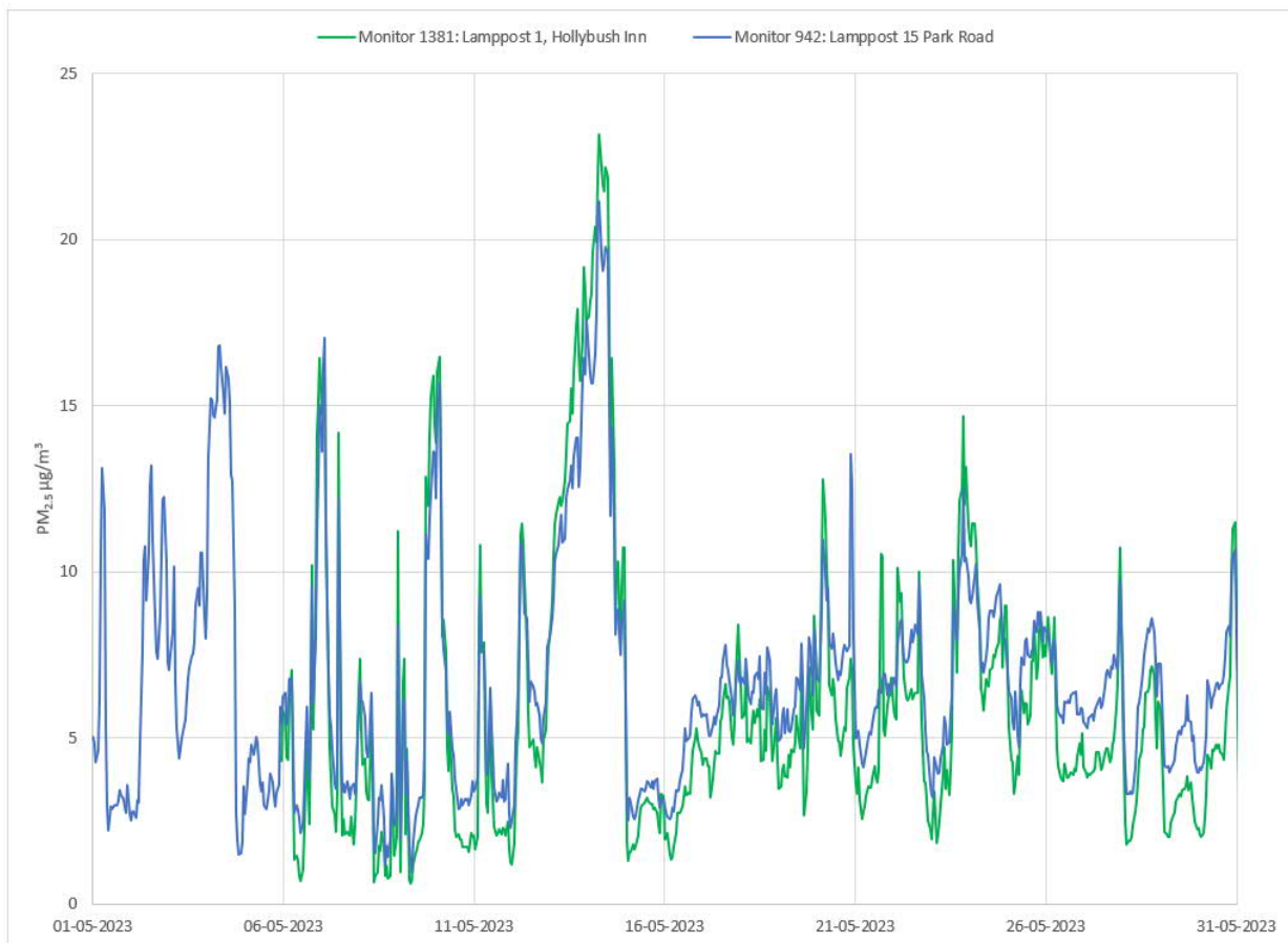
Figure 5 - Monitored Zephyr PM 2.5 Hourly Concentrations (µg/m 3 )
