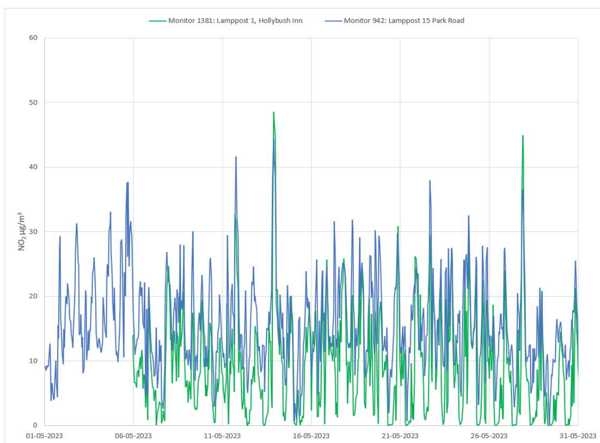
Figure 3 - Monitored Zephyr NO 2 Hourly Concentrations (µg/m 3 )
